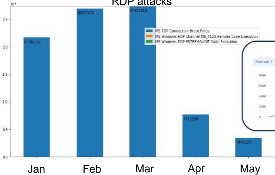
RDP attacks
